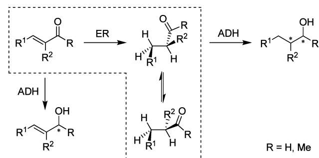
Figure 3. Typical chemical path of \alpha,\beta -unsaturated aldehyde/ketone reductions, with isolated enzymes or microorganisms.
