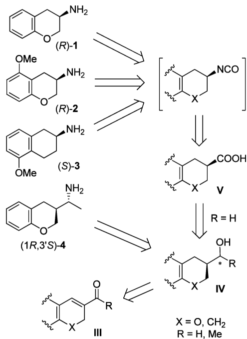
Figure 2. Retrosynthesis of amines 1–4.
