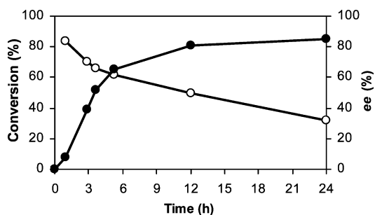
Figure 4. Progress curve of the biotransformation of 6a into ( S )-6b by OYE2 (conversion (●), ee (○)). Experimental conditions: 10 g L -1 of substrate (loaded on 10 g L -1 resin), 150 μg mL -1 of OYE2, 4 U mL -1 of GDH, 4 equiv of glucose, 0.1 mM NADP + , 50 mM KP i buffer pH 7.0, 30 °C, 160 rpm.
