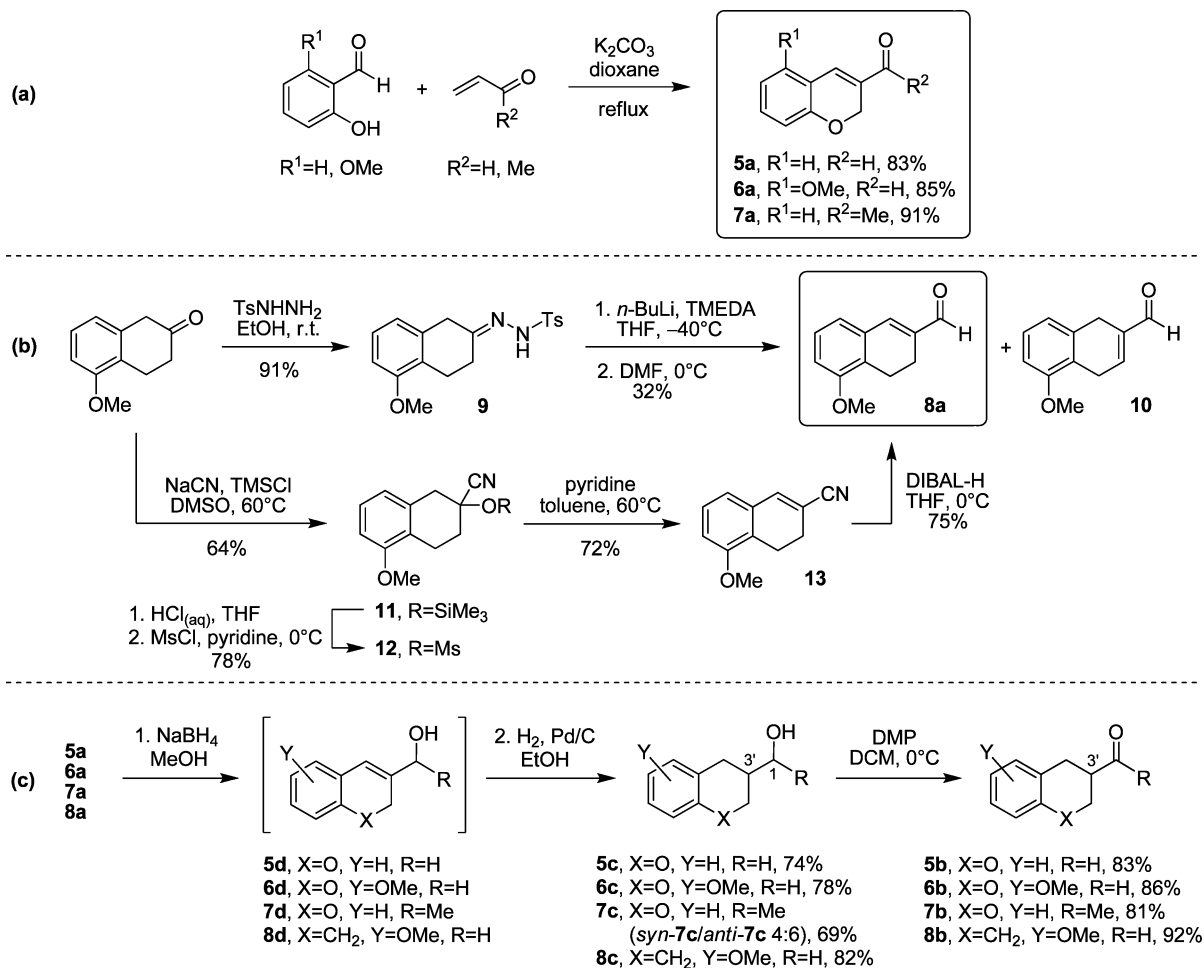
Scheme 1. Synthesis of Substrates 5a–8a and Reference Racemic Materials 5b–8b and 5c–8c
